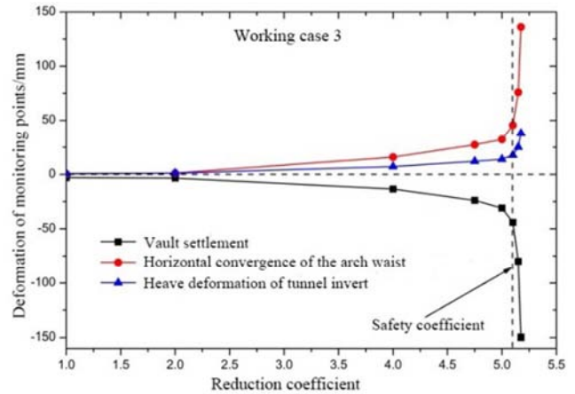
Figure 7. Curves of displacement with reduction factor in case 3.
