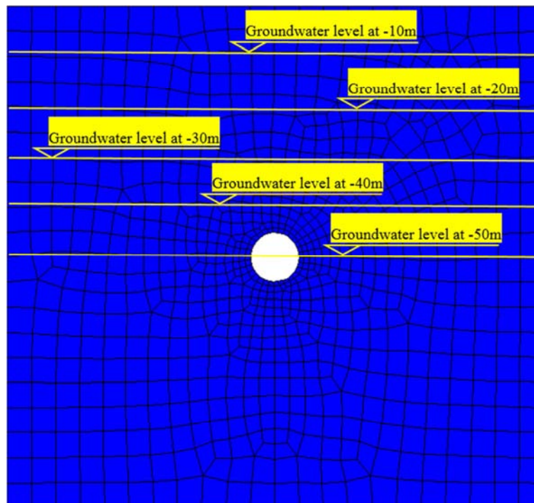
Figure 8. Relative position between groundwater level and tunnel.
