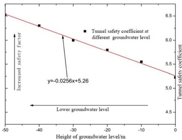
Figure 10. Curves of safety factor with groundwater level.
