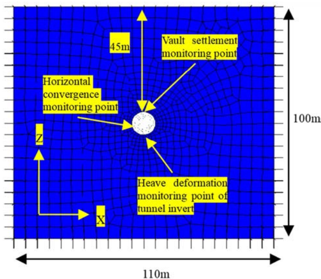
Figure 2. The numerical model.
